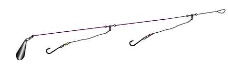
SURFCASTING RIG Hook size 1, length 160cm, line 0.60/0.35mm.
