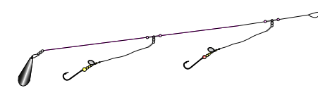
SURFCASTING RIG Hook size 1, length 120cm, line 0.60/0.35mm.
