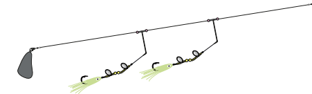
NATURAL BAIT RIG Hook size 1, length 100cm, line 0.60/0.50mm.
