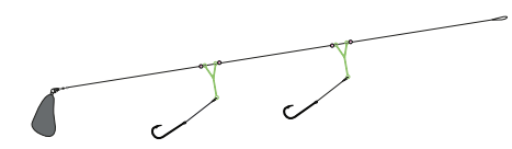
NATURAL BAIT RIG Hook size 1, length 95cm, line 0.50/0.50mm.
