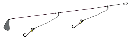
NATURAL BAIT RIG Hook size 1, length 115cm, line 0,60/0.40mm.
