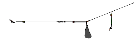
NATURAL BAIT RIG Hook size 1, length 95cm, line 0.60/0.40mm.
