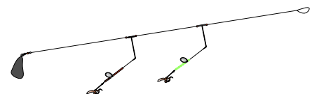
NATURAL BAIT RIG Hook size 1, length 85cm, line 0.60/0.40mm.
