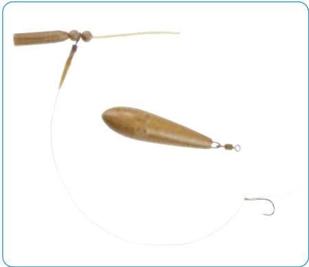
HELICOPTER DISTANCE RIG, HOOK SIZE 4
